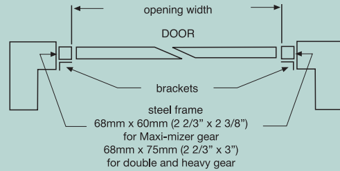
Fitting to Wessex steel retractable frame, within the brickwork aperture.
